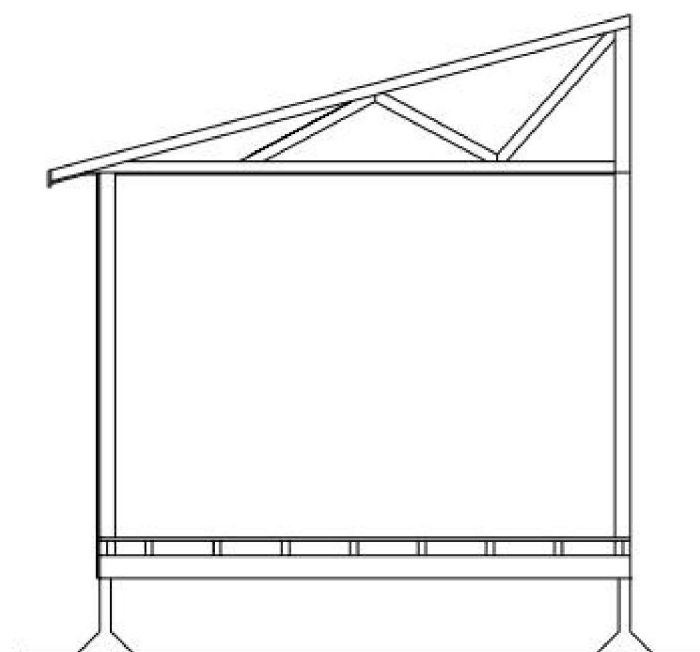
Section - mono-pitched
